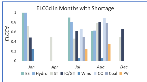
Figure 5. ELCCd values in shortage event periods categorized by unit type. ST : Steam Turbine, ES : Energy Storage, CC : Combined Cycle
